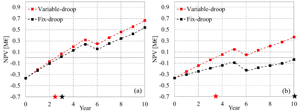
Figure 8.12 Estimated NPV trends and pay back time with variable-droop or fix-droop strategies; Two valorisations of LoR are assumed: (a) p_{LoR} = 140 \text{ €/MWh} , (b) p_{LoR} = 500 \text{ €/MWh}
