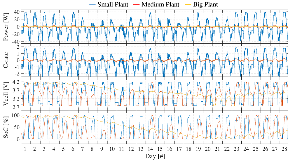
Figure 9.14 Simulation results for the month of February of year 1 with the electrical model M3: Power profile, C-rate profile, Voltage and estimated SoC for the hypotheses of Table 9.5
