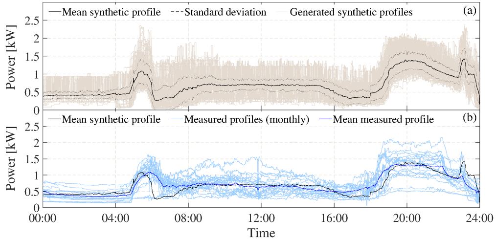
Figure 9.9 (a) Synthetic load profiles (grey), mean synthetic profile (solid-black) and standard deviation (dotted-black); (b) Comparison between the mean synthetic profile (black), measured monthly average profiles (light blue) and average measured profile (blue)
